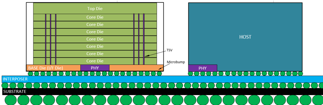
Figure 2: High-Bandwidth Memory Leverages Stacked Memory Components for Density and High I/O Counts
